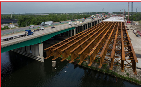
I-294 Mile Long Bridge
